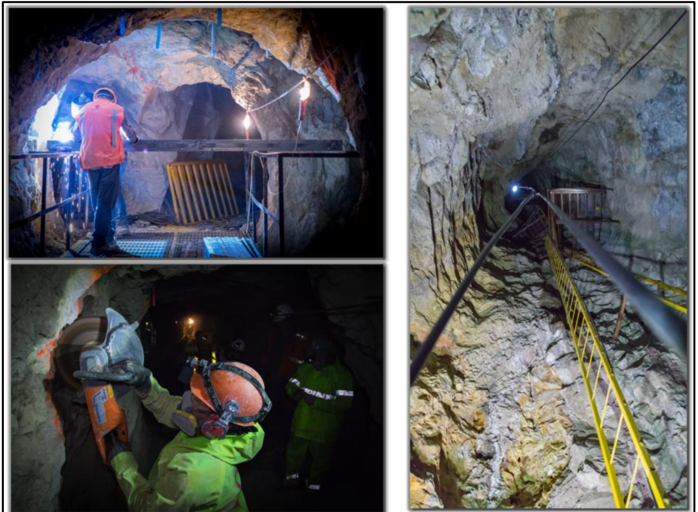
Figure 9-1: Photos of Las Chispas Underground Rehabilitation Activities
