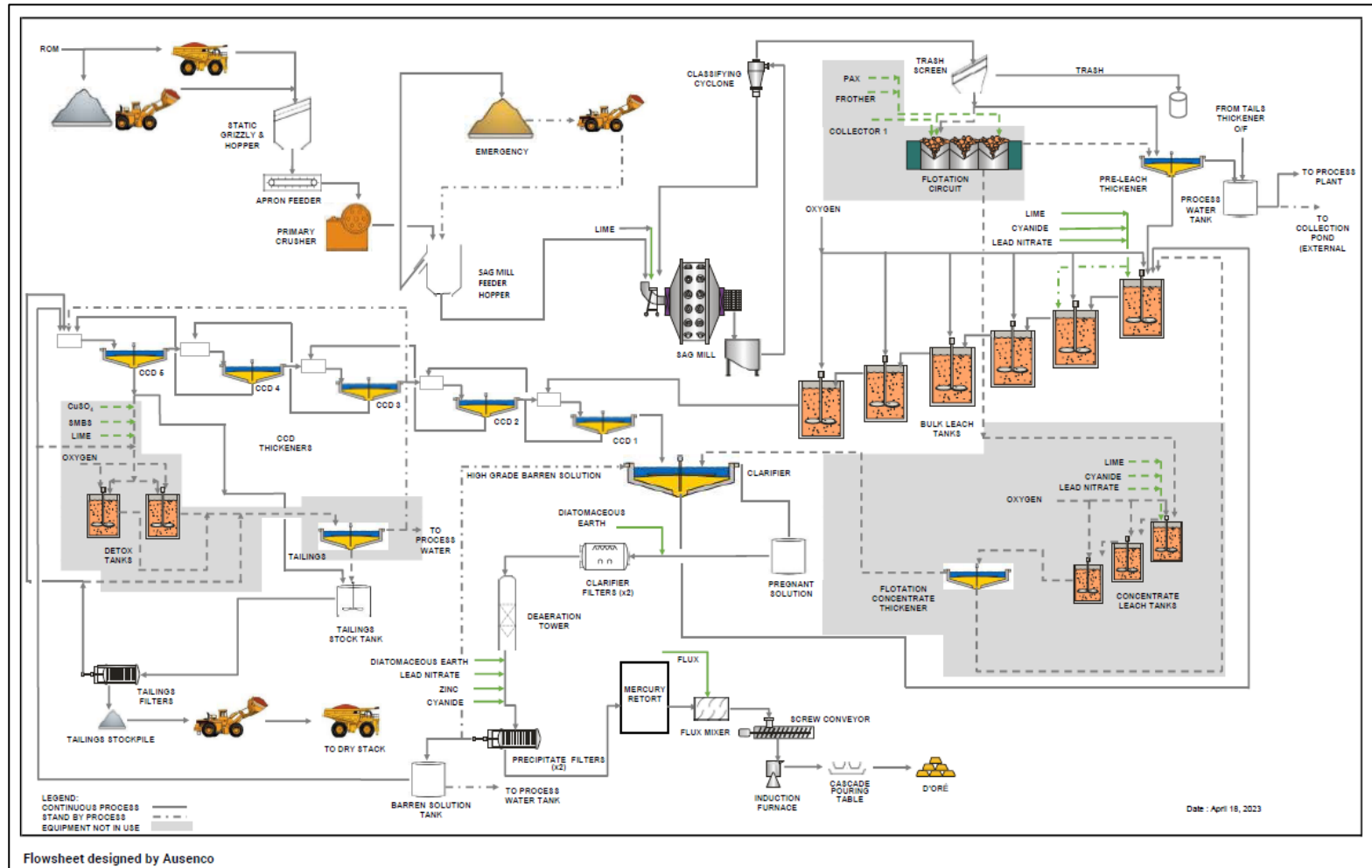
Figure 17-2: Overall Process Flow Diagram
