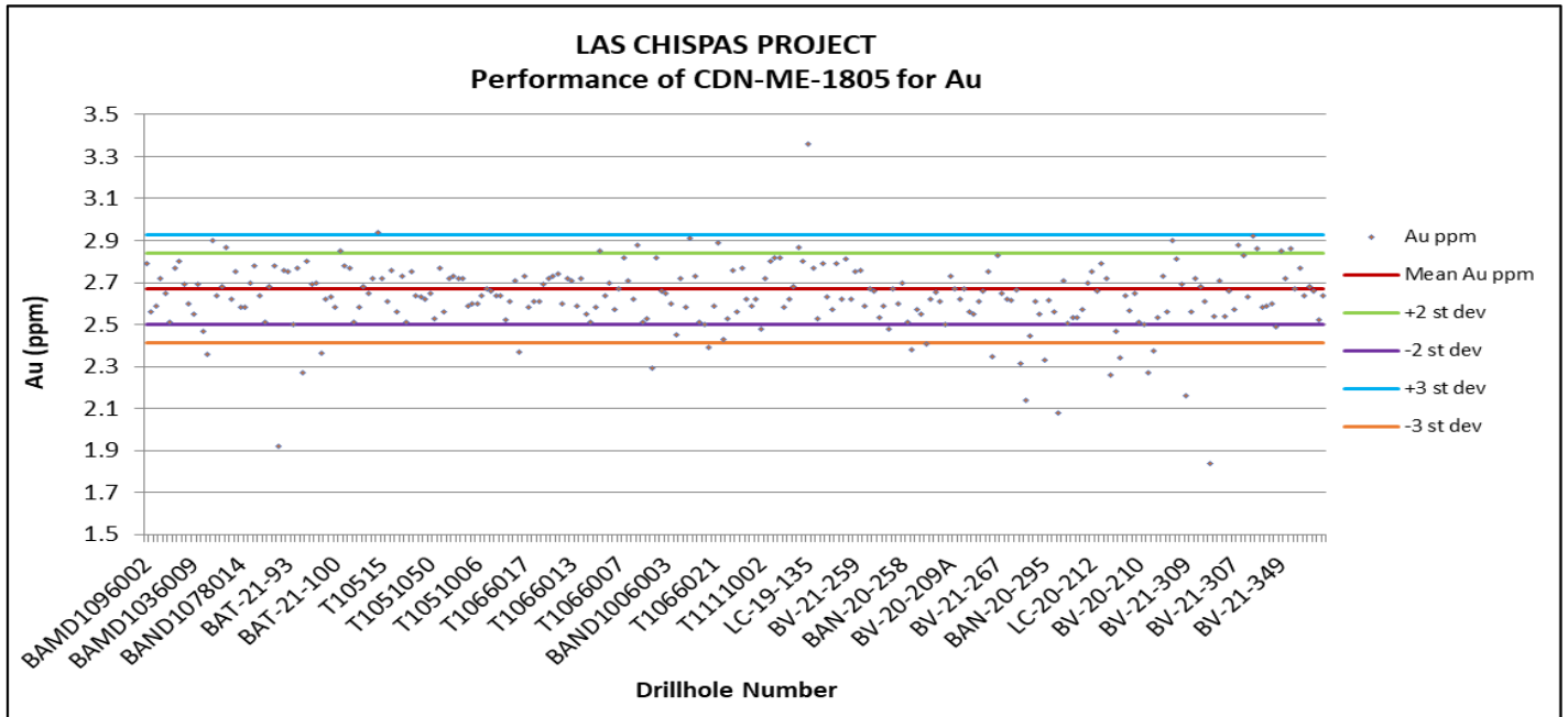
Figure 11-1: CRM CDN-ME-1805 Analysis, Gold
