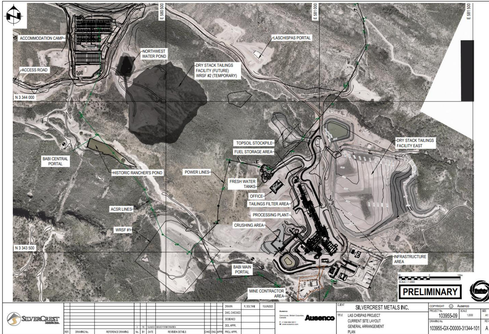
Figure 1-4: Site Layout
