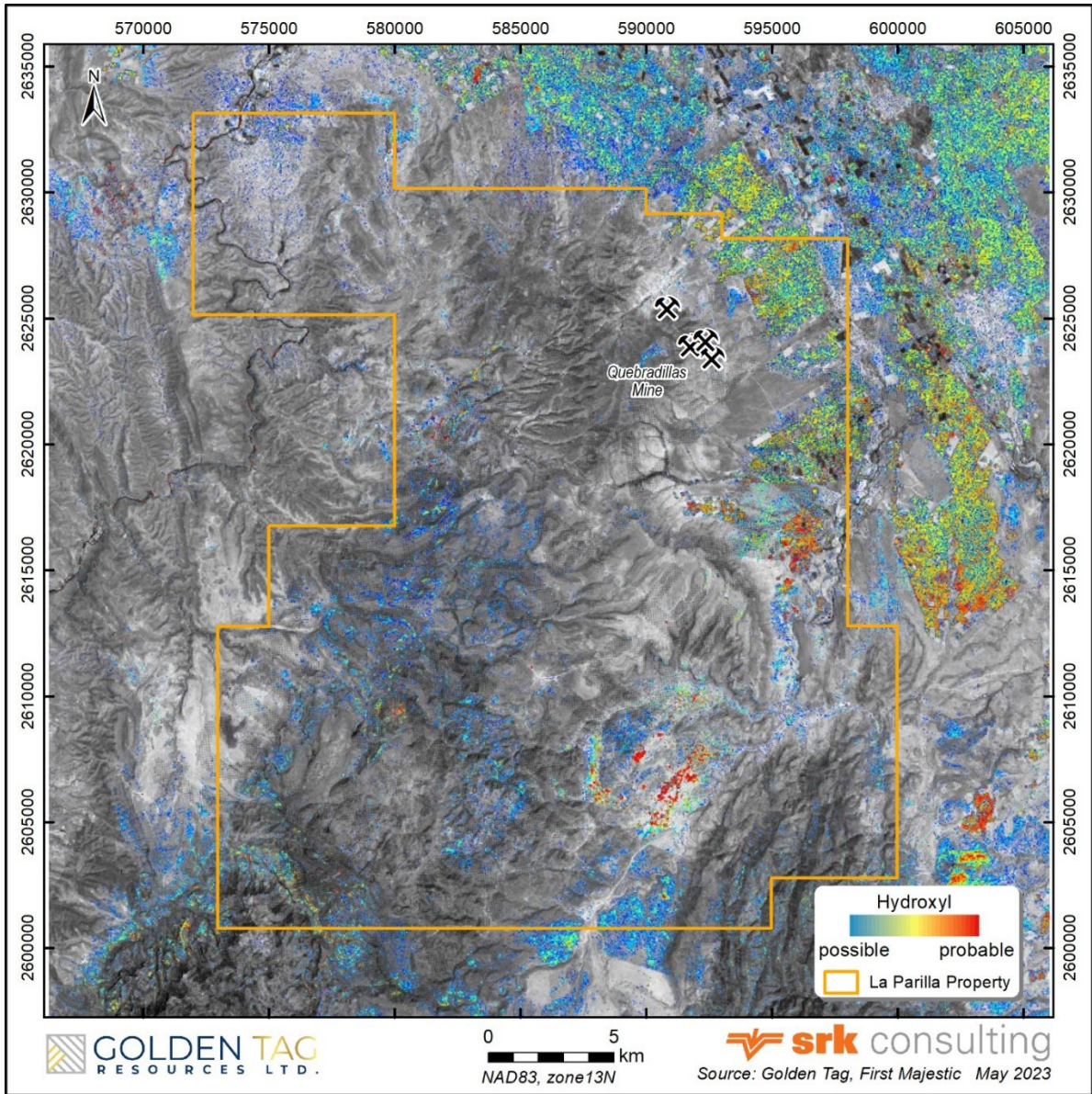
Figure 5-10: Hydroxyl (Total Intensity) Alteration Map from the 2019 PhotoSat Alteration Mapping Program (Modified after PhotoSat Information LTd., 2019)
