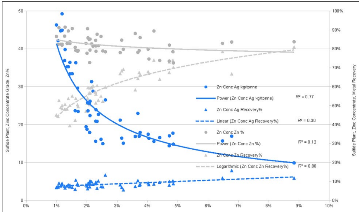
Figure 12-15: La Parrilla Zinc Circuit, Recovery and Grade versus Mass Pull (FMS 2023)
